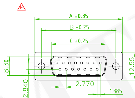
57MDSSXM-XXNHG0XA-01 Front rivet #4-40 height=5.8
