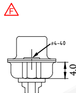
57MDSSXM-XXNFG0XA-01 Rear rivet #4-40 height=4.0
