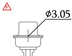
57MDSSXM-XXNNG0XA-01 Clear Hole
