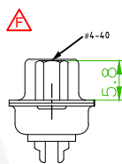
57MDSSXM-XXNHG0XA-01 Front rivet #4-40 height=5.8
