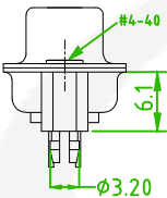
THREAD INSERT #4-40 57MDDSM-XXBAXXX-10
