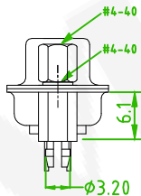
THREAD INSERT #4-40 +JACK SCREW #4-40 REMOVABLE 57MDDSM-XXCCXXXX-10
