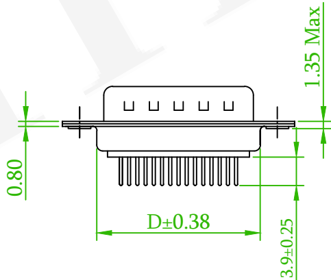
THREAD INSERT #4-40 +JACK SCREW #4-40 REMOVABLE 57MDDSM-XXCCXXXX-10
