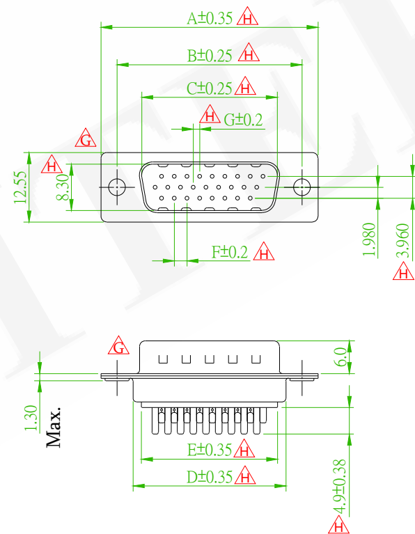
N: Clear Hole Ø3.05mm 57HDSSXM-XXNNXXXA-01
