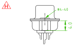
Rear Rivet #4-40, H=4.0 57HDSSXM-XXNFXXXA-01
