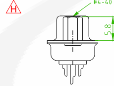
Front Rivet #4-40, H=5.8 57HDSSXM-XXNHXXXA-01
