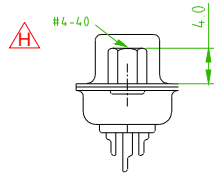
Front Rivet #4-40, H=4.0 57HDSSXM-XXNDXXXA-01
