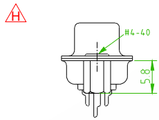
Rear Rivet #4-40, H=5.8 57HDSSXM-XXNIXXA-01
