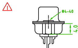
Rear Rivet #4-40, H=4.0 57HDSSXF-XXNFXXA-01
