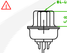
Front Rivet #4-40, H=5.8 57HDSSXF-XXNHXXA-01
