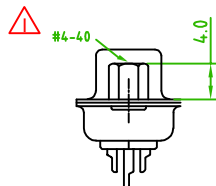
Front Rivet #4-40, H=4.0 57HDSSXF-XXNDXXA-01
