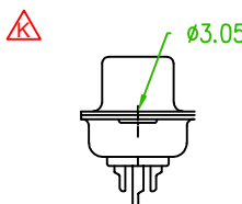
Clear Hole Ø3.05mm 57HDSSXF-XXNNXXA-01
