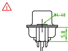
Rear Rivet #4-40, H=5.8 57HDSSXF-XXNIXXA-01
