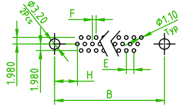
Re Layout P.C.B. 26 /44 /62 POSITION
