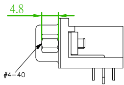
57HDDR XM-XXACXXXX-01 THREAD INSERT #4-40 + JACK SCREW #4-40 REMOVABLE
