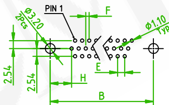
RECOMMENDED PCB LAYOUT 26/44/62 POSITION (PCB TOLERANCE ±0.05)
