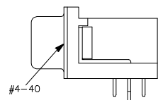
57HDDR XM-XXAAXXXX-01 THREAD INSERT #4-40
