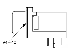
57HDDR XM-XXABXXXX-01 THREAD INSERT #4-40 + JACK SCREW #4-40 ATTACHED
