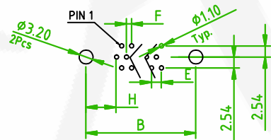
RECOMMENDED PCB LAYOUT 15 POSITION (PCB TOLERANCE ±0.05)
