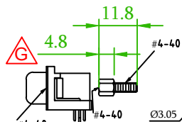
57DBDRXA-XXABXXXX-01 THREAD INSERT #4-40 + JACK SCREW #4-40 ATTACHED
