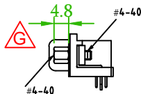
57DBDRXA-XXACXXXX-01 THREAD INSERT #4-40 + JACK SCREW #4-40 REMOVABLE + RIVET GROUND STRAP
