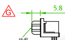
57DBDRXA-XXABXXXX-01 THREAD INSERT #4-40 + JACK SCREW #4-40 ATTACHED
