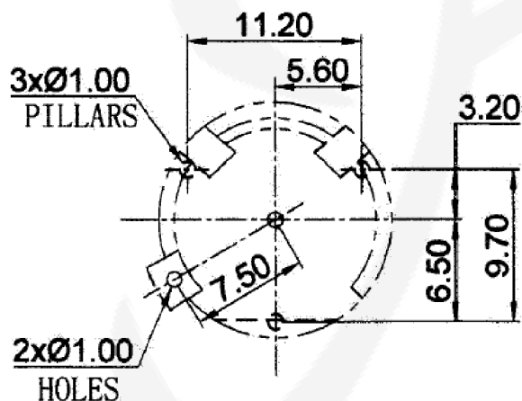
PCB MOUNTING LAYOUT
