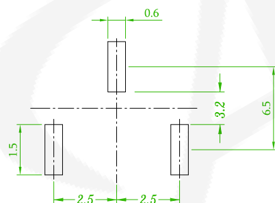
Recommended PCB Layout (PCB TOLERANCE ±0.1)
