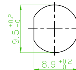
RECOMMENDED MOUNTING HOLE MAXIMUM PANEL THICKNESS:5.5MM
