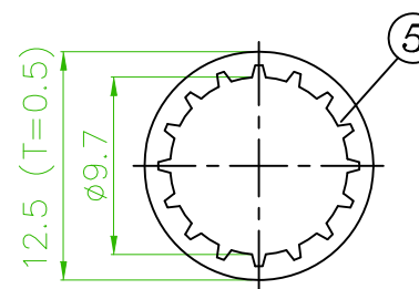
WASHER
