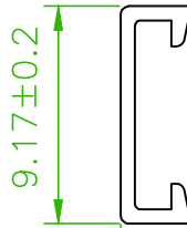
5W5082D0-104T0WBLA01-CV-1 (Through type)
