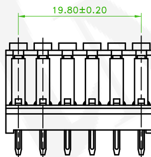
1x6 PIN
