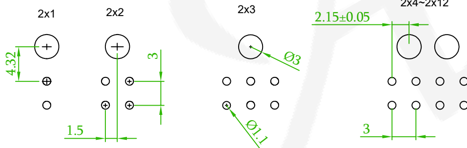
Recommended PCB Layout (PCB TOLERANCE \pm 0.1 )
