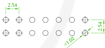
Recommended P.C.B Layout (PCB BOARD TOLERANCE±0.05)
