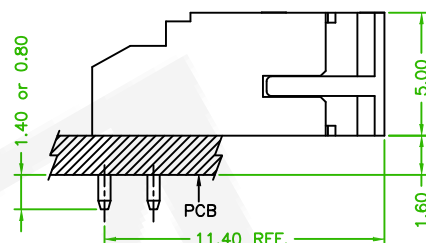
MATED CONDITION
