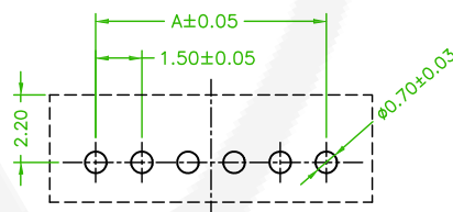
P.C.B. LAYOUT (TOP VIEW)
