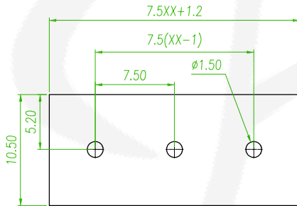
Recommended PCB Layout (PCB TOLERANCE ±0.1)
