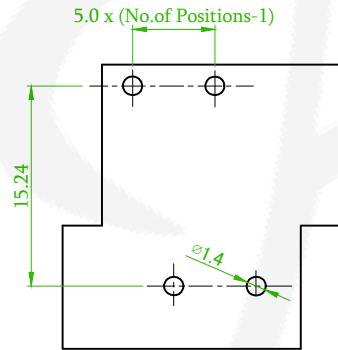
Rrcommmed P.C.B Layout (PCB TOLERANCE±0.1)
