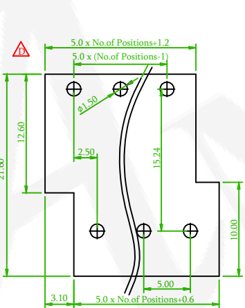
Recommended P.C.B Layout (PCB TOLERANCE±0.1)
