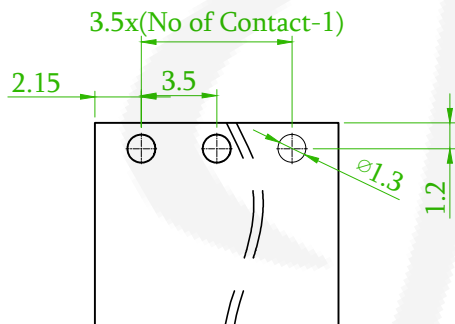
P.C.B LAYOUT TOLERANCE±0.1
