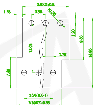
Recommended PCB Layout (PCB TOLERANCE ±0.1)
