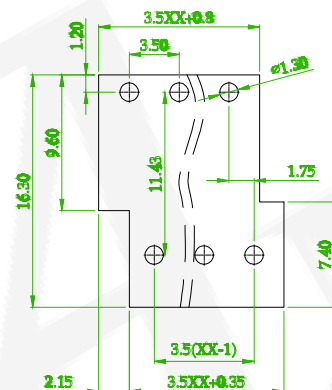
Recommended PCB Layout (PCB TOLERANCE ±0.1)
