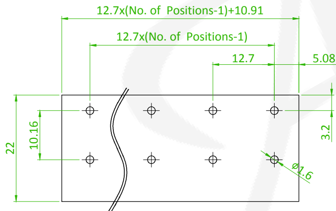
Recommended P.C.B Layout (PCB TOLERANCE ±0.1)
