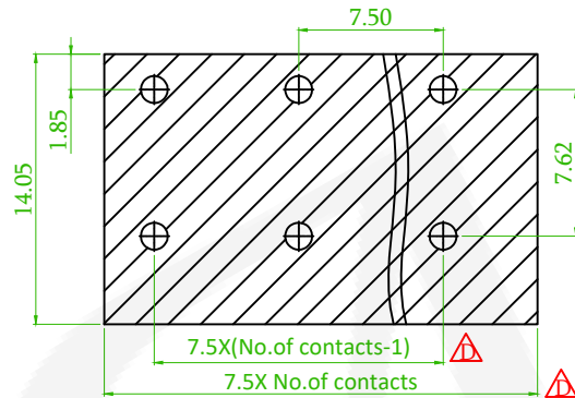
Recommended PCB Layout (PCB TOLERANCE \pm 0.05 )
