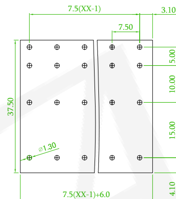
Recommended PCB Layout (PCB TOLERANCE ±0.05)
