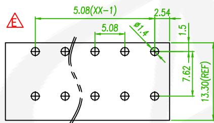
Recommended PCB Layout (PCB TOLERANCE \pm 0.05 )
