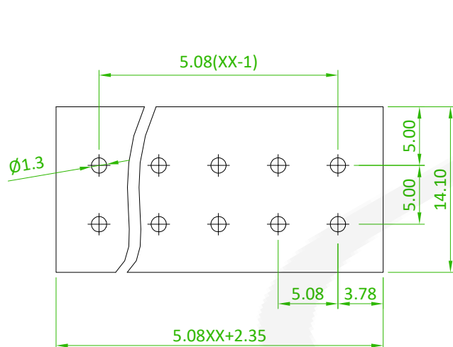
Recommended PCB Layout (PCB TOLERANCE \pm 0.05 )
