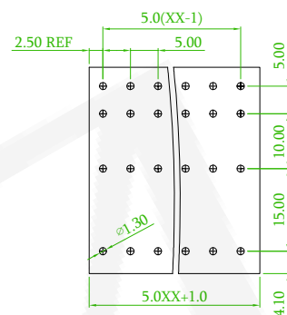
Recommended PCB Layout (PCB TOLERANCE \pm 0.05 )
