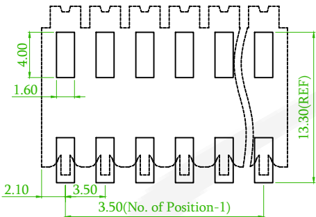
Rrcommened P.C.B Layout (PCB TOLERANCE±0.05)
