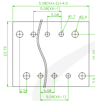
Recommended PCB Layout (PCB TOLERANCE \pm 0.05 )
