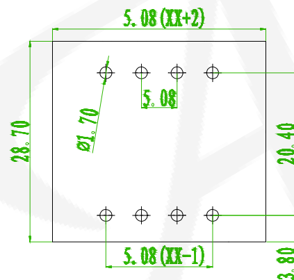
PCB LAYOUT
