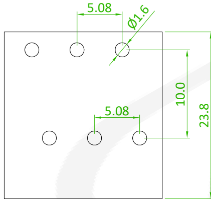
Recommended PCB Layout (PCB TOLERANCE \pm 0.05 )
