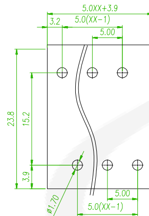
Recommended PCB Layout (PCB TOLERANCE \pm 0.05 )
