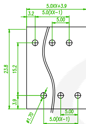
PCB LAYOUT
