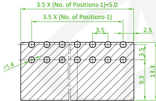
P.C.B LAYOUT TOLARANCES±0.1
