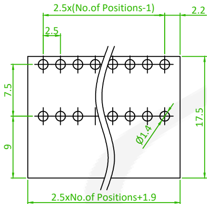
Recommended PCB Layout (PCB TOLERANCE ±0.1)
