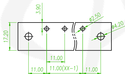
RECOMMENDED PCB LAYOUT (PCB TOLERANCE \pm 0.05 )
