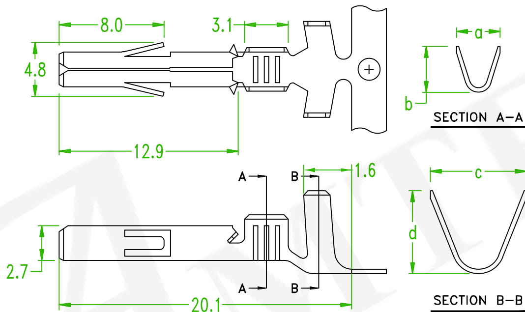
Ordering & Dimensional Information ( mm )
