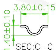
SEC:C-C
