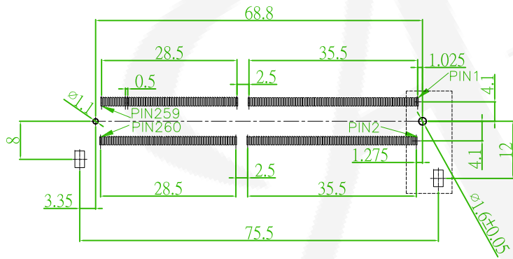
PCB LAYOUT TOLERANCE ±0.1
