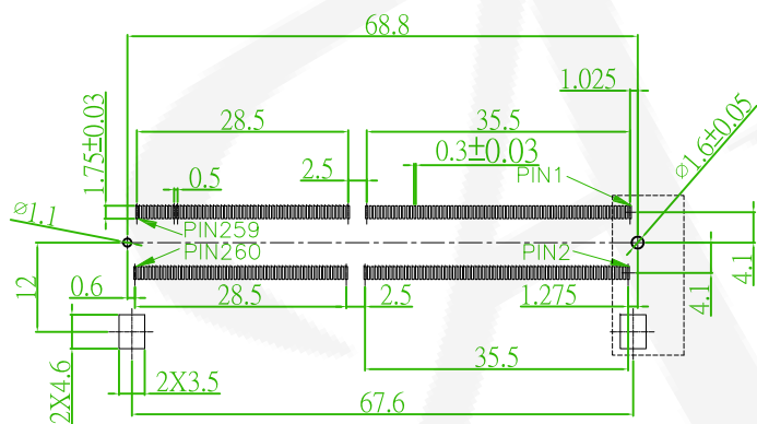
PCB LAYOUT TOLERANCE ±0.1
