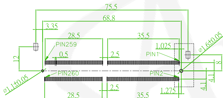
PCB LAYOUT TOLERANCE \pm 0.1
