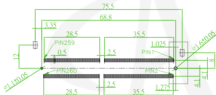
PCB LAYOUT TOLERANCE ±0.1
