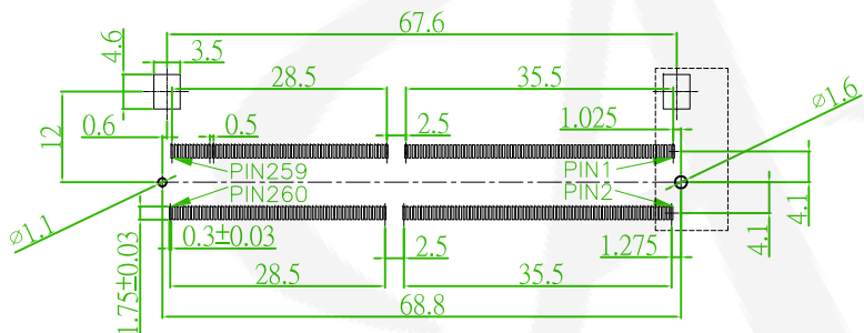
PCB LAYOUT TOLERANCE ±0.1
