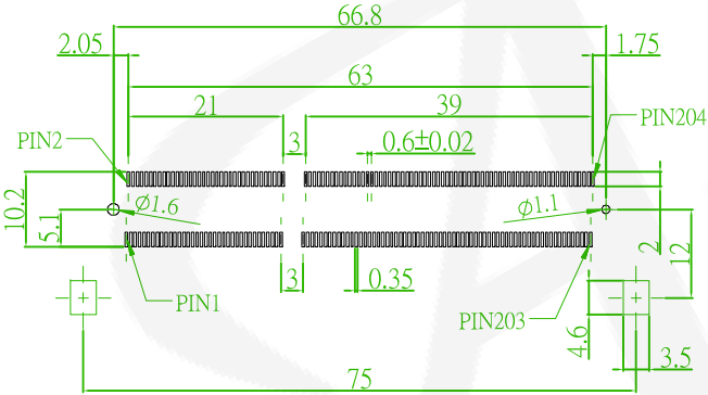
PCB LAYOUT : TOLERANCE ±0.1
