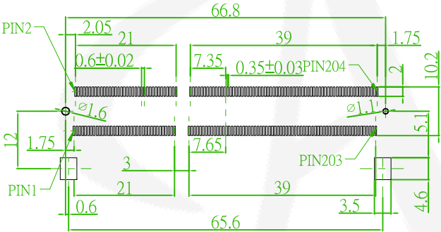
PCB LAYOUT : TOLERANCE ±0.1
