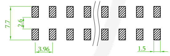
Recommended PCB Layout (PCB TOLERANCE ±0.1)
