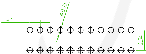
Recommended PCB Layout (PCB TOLERANCE ±0.1)
