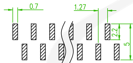
A Type
