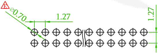
Recommended PCB Layout (PCB TOLERANCE ±0.05)
